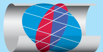
Multi-path measuring arrangement with crossed paths
